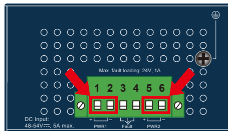
Figure 3-3: Industrial PoE++ Switch DC Input
