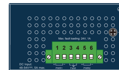
Figure 3-2: Industrial PoE++ Switch Upper Panel
